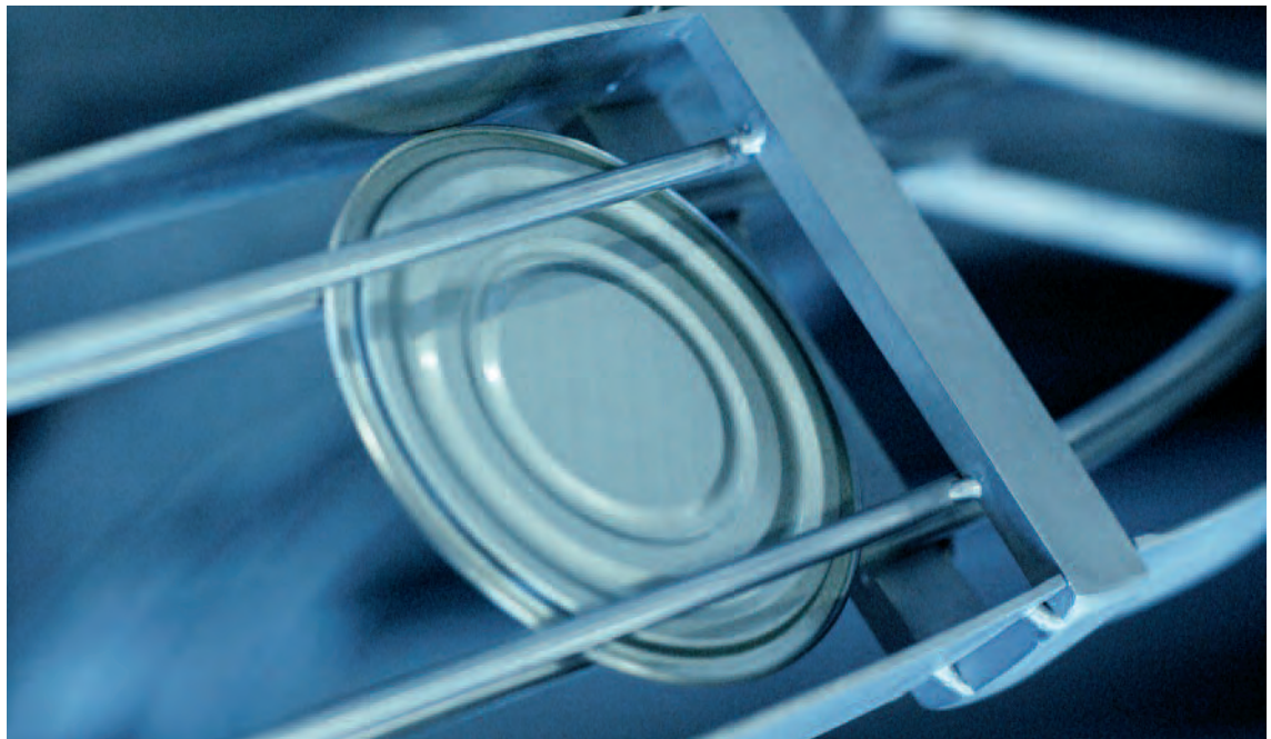
TRANSFERRING ENDS FROM THE CURLING STATION TO THE COMPOUND LINER
